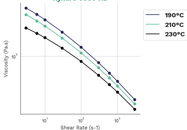
Viscosity-shear rate Kynar® 9000 HD
